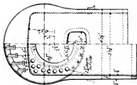
Fig. 5113. Section at Firebox of Water Tube Locomotive Boiler. London & South Western.
